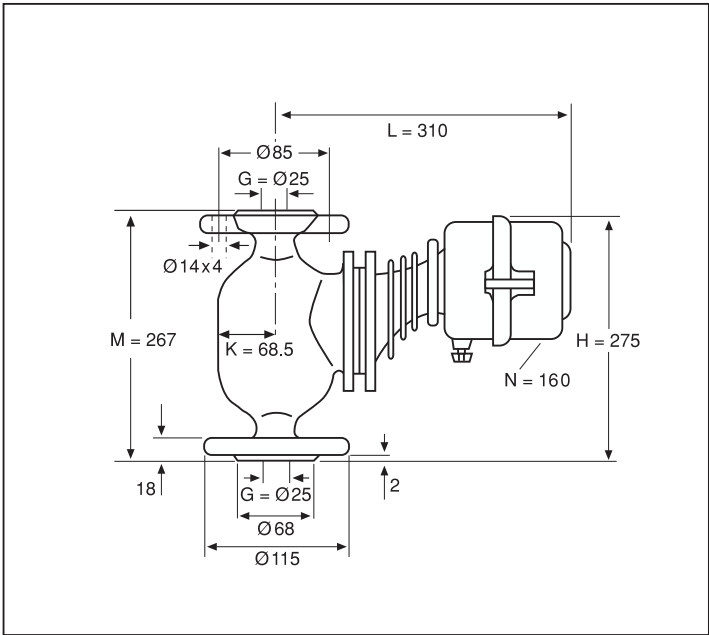
FLANGED BODY
